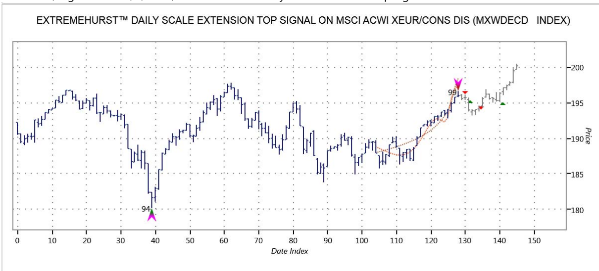
Chart #24, Signal Date: 6/9/2014, ExtremeHurst™ daily scale Extension Top signal on MXWDECD Index
