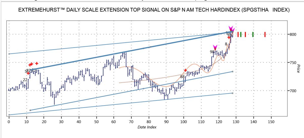
Chart #19, Signal Date: 7/2/2014, ExtremeHurst™ daily scale Extension Top signal on SPGSTIHA Index
