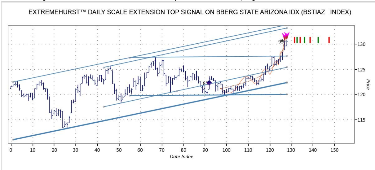
Chart #10, Signal Date: 7/2/2014, ExtremeHurst™ daily scale Extension Top signal on BSTIAZ Index
