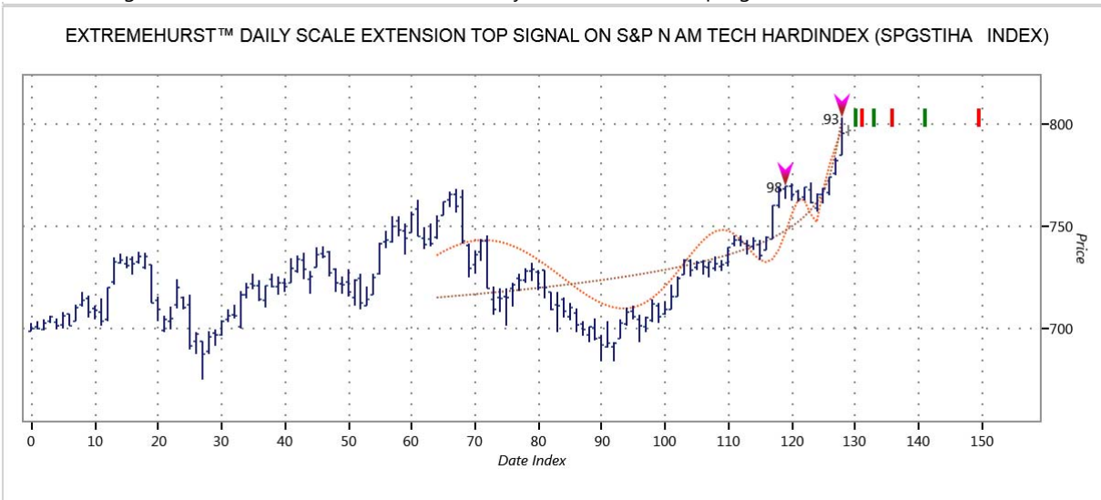
Chart #28, Signal Date: 7/1/2014, ExtremeHurst™ daily scale Extension Top signal on SPGSTIHA Index
